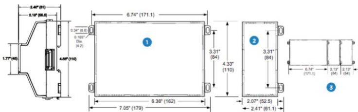
Compatible with (DIN43880) enclosures Suitable for mounting to a panel or to an EN50022 standard 35mm rail
